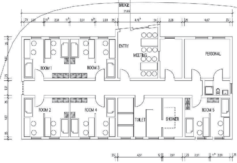
CHILDREN'S HOUSE SECOND FLOOR
