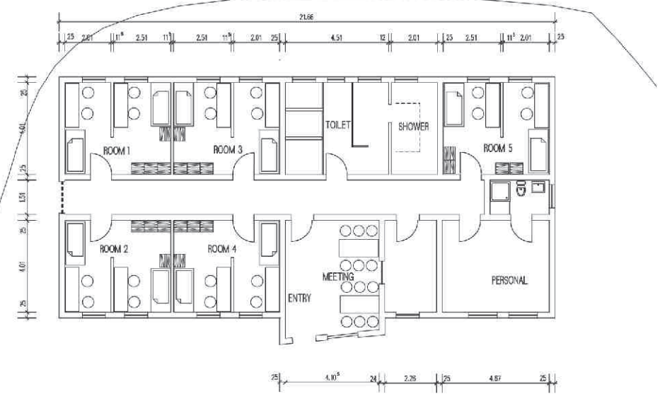
CHILDREN'S HOUSE FIRST FLOOR
